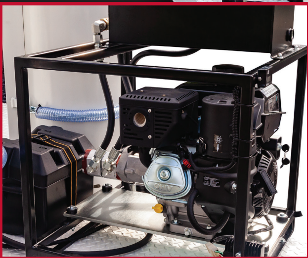
Powerful 9.5 hp Kohler engine certified for and meets both EPA & CARB regulations
