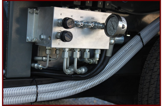
ENGINEERED HYDRAULIC SYSTEMS AND MANIFOLDS
