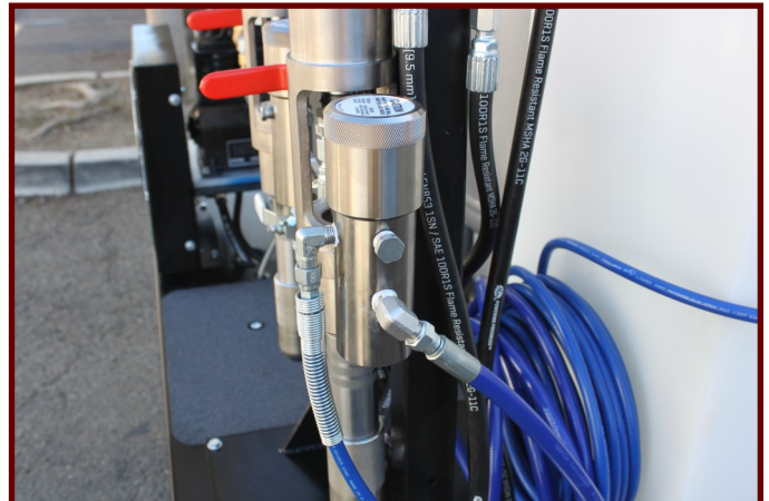
HIGH PRESSURE PAINT FILTER AT EACH PUMP OUTLET
