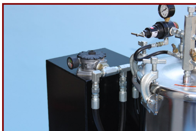
HYDRAULIC TANK WITH SIGHT GAUGE AND FILTER
