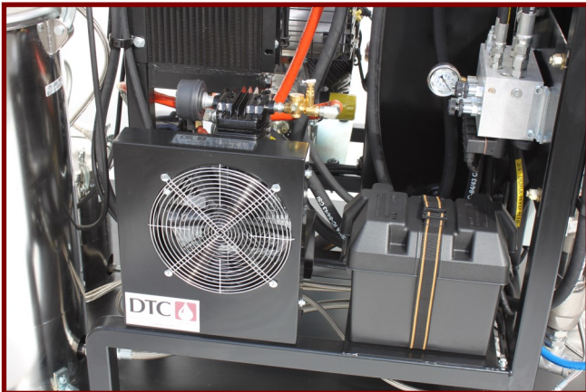
HYDRAULICALLY OPERATED AIR COMPRESSOR
