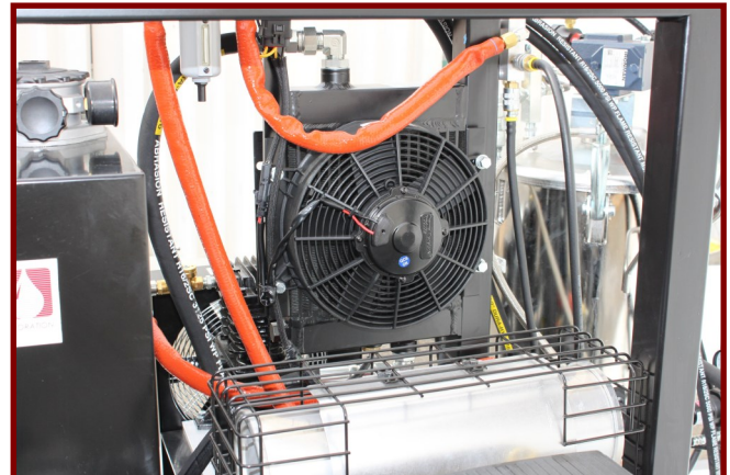
HYD OIL COOLER FOR EFFICIENT OPERATION
