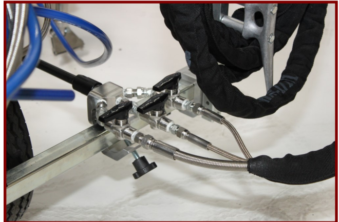
INTEGRATED MIX MANIFOLD WITH SS BALL VALVES
