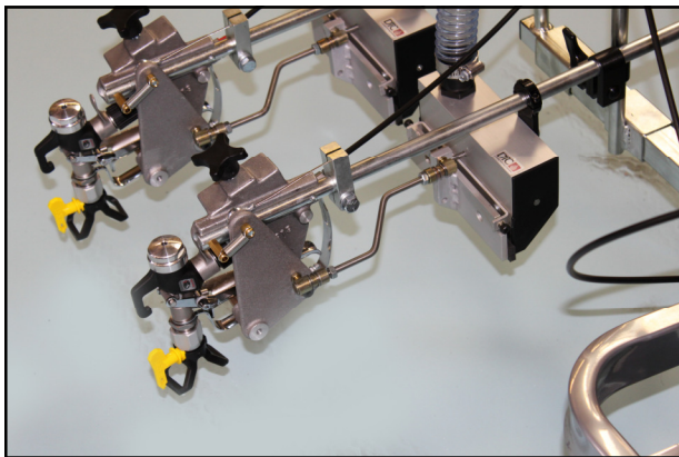
Quick connect swivel fittings and linkage provide ease of installation and removal when painting lines where beads are not needed.
