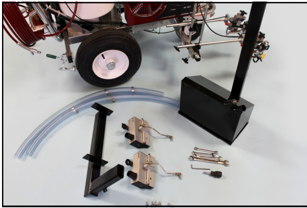
Kits come complete with hopper, dispensers, hoses and all mounting hardware required for operation (tools not included)
