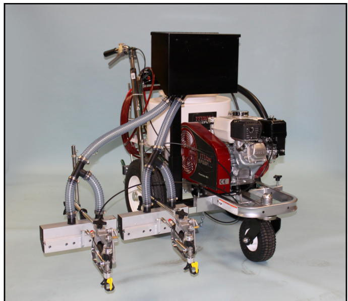
Flow of beads is controlled by adjusting the slide plate opening behind door. Dual plates allow selecting 4" or 6" width
