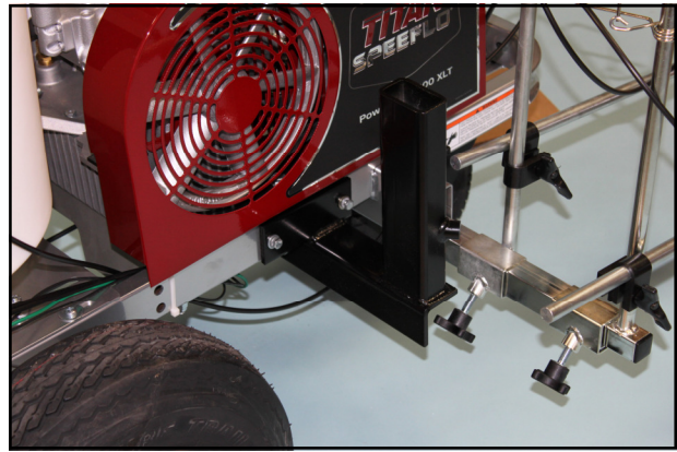
Pre-drilled and tapped holes in frame make mounting the bead hopper very easy. Durable powder coated hopper and mounting brackets
