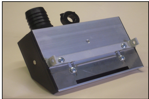
Flow of beads is controlled by adjusting the slide plate opening behind door. Dual plates allow selecting 4" or 6" width
