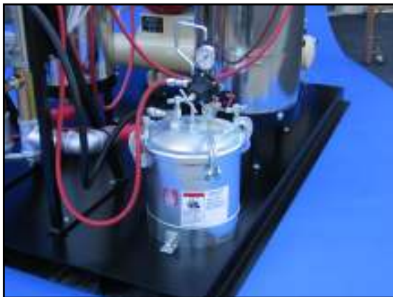
Optional solvent flushing system is available that allows static mixer to be reused by purging epoxy prior to setting up
